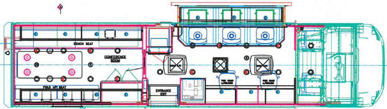
FLOOR PLAN
